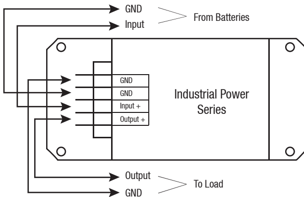
4 Terminal Type, No Remote Control
