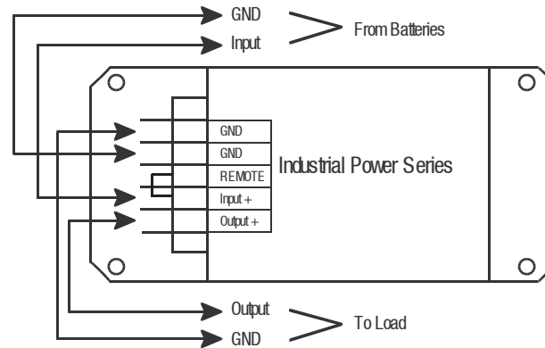
5 Terminal Type, With Remote ON/OFF Control
