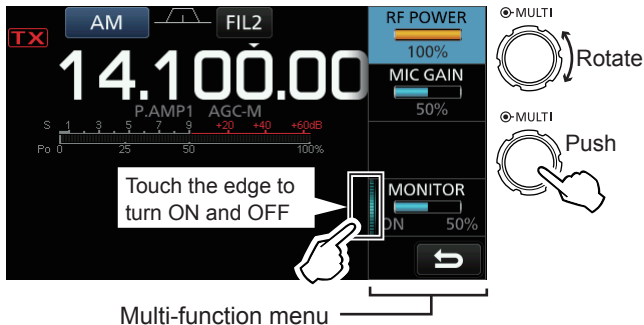
Multi-function menu
