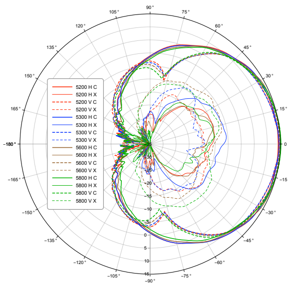
5 GHz Azimuth
