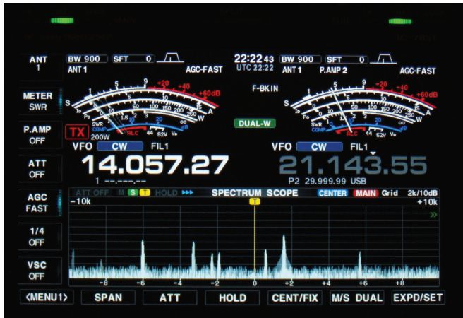
Figure 2 — A view of the front panel display of the IC-7851 during CW operation. Note that both receivers are active on different bands and the spectrum display is showing \pm 10 kHz around the operating frequency of the main receiver. Note particularly the S meters — they are digital images that look just like real moving-coil D'Arsonval meter movements.
