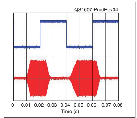
Figure 4 — CW keying waveform for the Icom IC-7851 showing the first two dits using external keying. Equivalent keying speed is 60 WPM. The upper trace is the actual key closure; the lower trace is the RF envelope. (Note that the first key closure starts at the left edge of the figure.) Horizontal divisions are 10 ms. The transceiver was being operated at 190 W output on the 14 MHz band.
