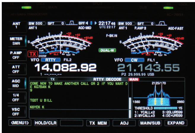
Figure 7 — The display during RTTY operation. Note the window on the lower right that provides tuning information by comparing the received spectrum to the RTTY mark and space frequencies. On the lower left is a screen portion with up to eight lines of decoded receive text. Below that is a space for a type-ahead buffer ready to send upon shift to transmit mode. Below the mini spectrum and waterfall displays are summaries of the first four transmit memories to allow sending via a keypad or connected keyboard. The transmit memories in detail can also be displayed on the lower portion of the screen to allow transmission via soft buttons, if the keypad or keyboard is not available.
