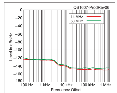
Figure 6 — Spectral display of the Icom IC-7851 transmitter output during phase noise testing. Power output is 190 W on the 14 MHz band (red trace) and 50 MHz band (green trace). The carrier, off the left edge of the plot, is not shown. This plot shows composite transmitted noise 100 Hz to 1 MHz from the carrier. The reference level is 0 dBc, and the vertical scale is in dBc/Hz.
