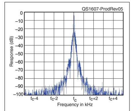
Figure 5 — Spectral display of the Icom IC-7851 transmitter during keying sideband testing. Equivalent keying speed is 60 WPM using external keying. Spectrum analyzer resolution bandwidth is 10 Hz, and the sweep time is 30 seconds. The transmitter was being operated at 190 W PEP output on the 14 MHz band, and this plot shows the transmitter output ±5 kHz from the carrier. The reference level is 0 dBc, and the vertical scale is 10 dB/division.
