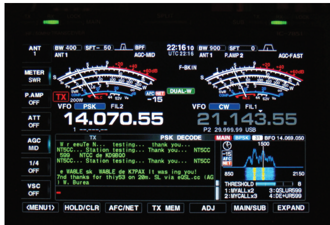
Figure 8 — Similar to Figure 7, but in PSK mode. The main differences are the additional PSK phase-indicating circle and the single center frequency. Each mode has its own set of recorded transmit messages.
