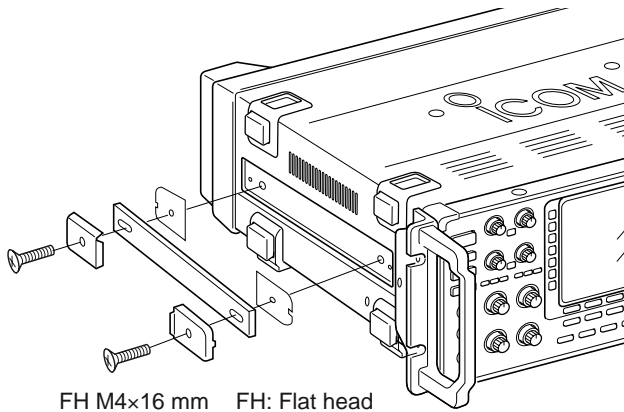
FH M4x16 mm FH: Flat head
