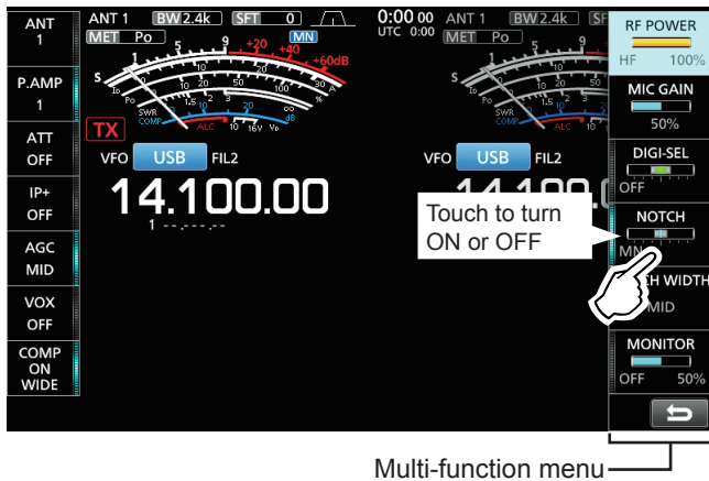
Multi-function menu
